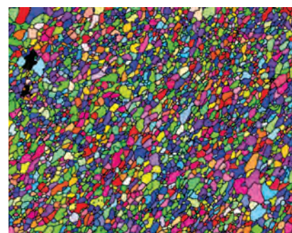
Fig. 3 — EBSD Thixomolded + thermomechanically processed + annealing: Grain Size – 2 μm, yield strength – 250 MPa, elongation – 12%, fatigue strength – 150 MPa, toughness – 28 MPam 0.5 , texture – MRD of 3.7 max. Courtesy of Tracy Berman.
