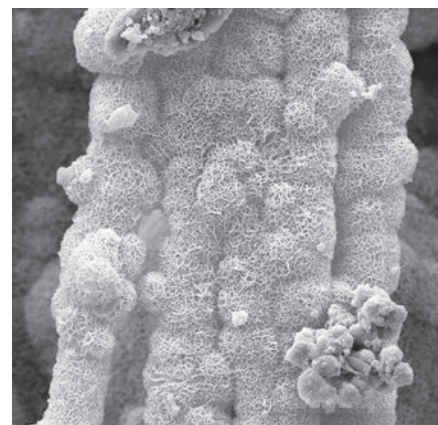
Self-Healing Concrete , the Electron Microscopy Prize winner of the University of Cambridge's annual photo contest. Courtesy of Tanvir Qureshi.
