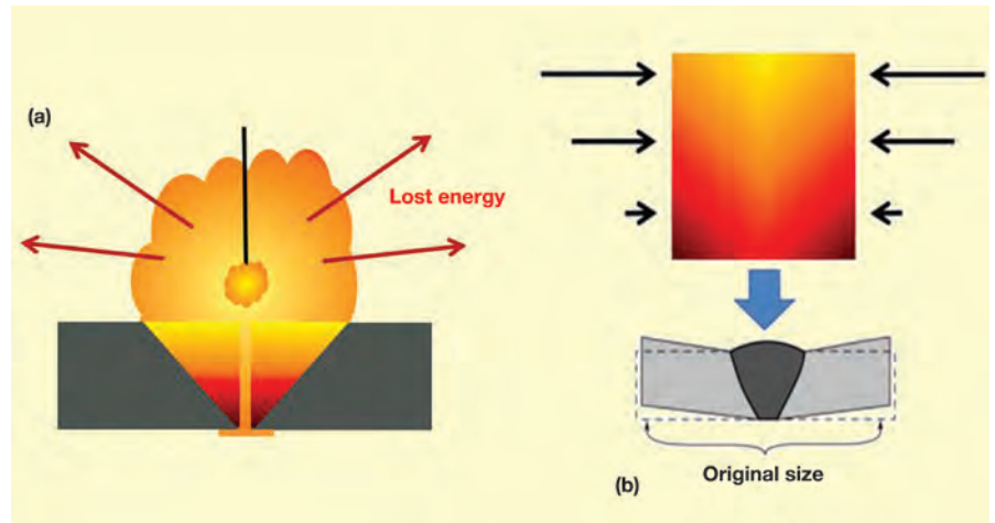
Fig. 2 — Arc welding distortion.
