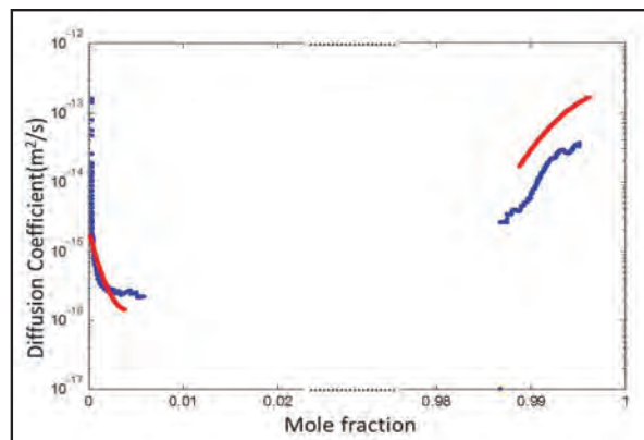
Fig. 2(b) — Comparison of interdiffusion coefficients obtained from the forward simulation [13] (red lines) with those obtained by the Sauer-Freize method [14] (blue lines).
