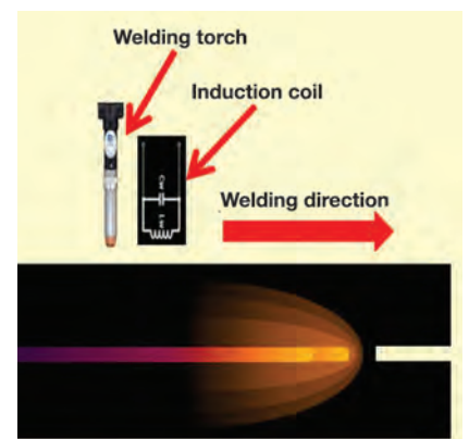
Fig. 1 — Schematic diagram of the HiDep welding process.
