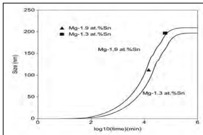
Fig. 4(b) — Predicted radius of Mg_2Sn precipitate in Mg-1.3 at% Sn and Mg-1.9 at% alloys along with experimental data [19] .
