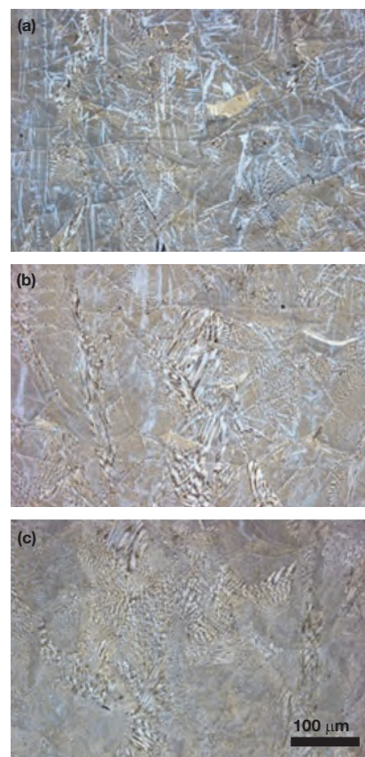
Fig. 2 — Effect of heat input on microstructure of as-built AISI 420 stainless steel: (a) Low heat input (P=200 W, v=1000 mm/s); (b) Moderate heat input (P=300 W, v=1000 mm/s); and (c) High heat input (P=300 W, v=800 mm/s).
