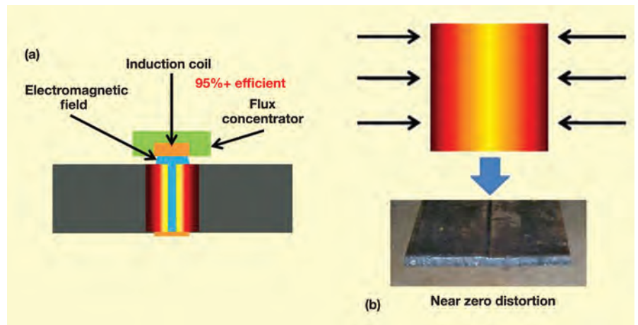
Fig. 3 — HiDep weld—low distortion.
